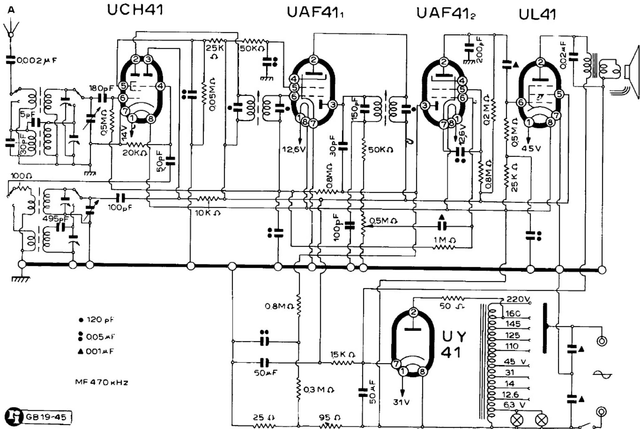
MINERVA RADIO - Mod 495/1
